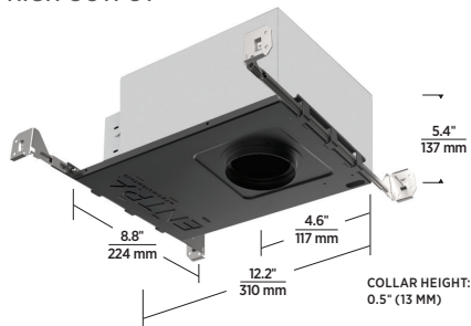
IC AIRTIGHT/FIRE-RATED CHICAGO PLENUM
