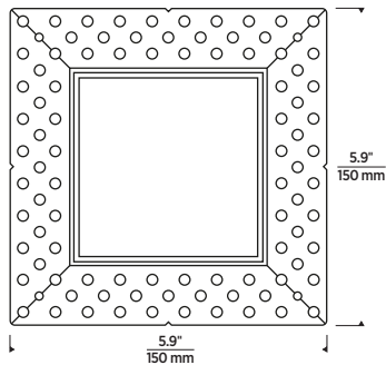
SQUARE DIE CAST (INCLUDED FOR FLANGELESS INSTALLATION)
