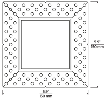
SQUARE DIE CAST (INCLUDED FOR FLANGELESS INSTALLATION)
