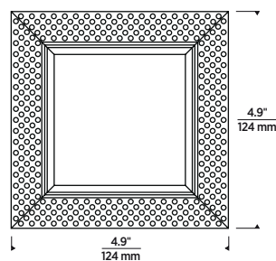
SQUARE SHEET METAL (OPTIONAL FOR FLANGELESS INSTALLATION)
