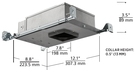
IC AIRTIGHT/FIRE-RATED/ CHICAGO PLENUM
