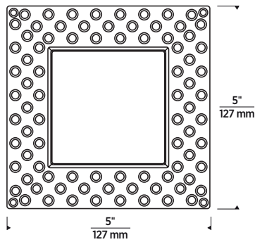
SQUARE DIE-CAST (INCLUDED FOR FLANGELESS INSTALLATION)
